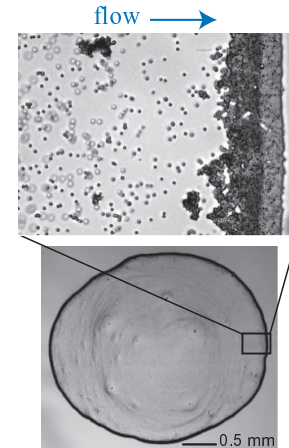
(b) particle deposition in suspension droplet
